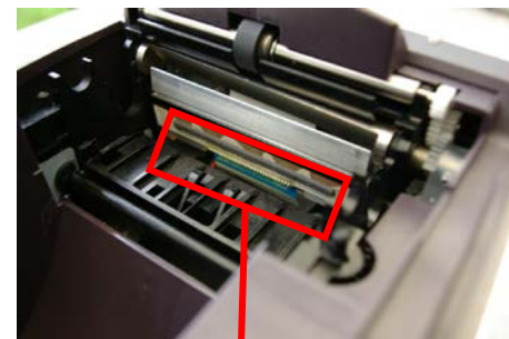
Clean Thermal Print Head with clean, dry cloth
